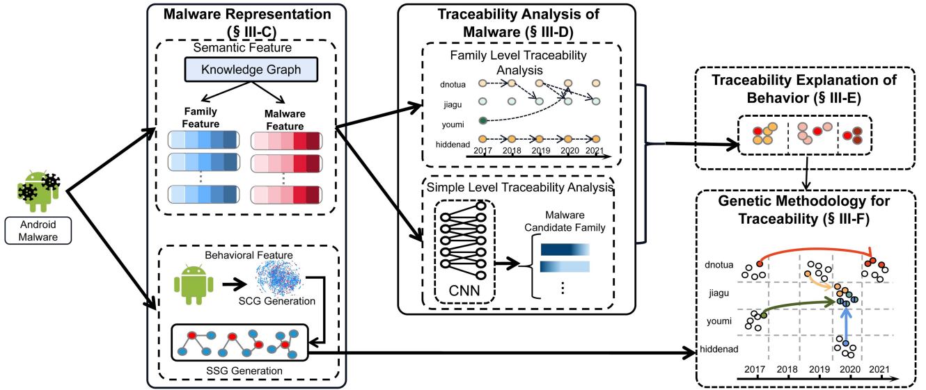
Fig. 2. The framework for malware traceability analysis.
