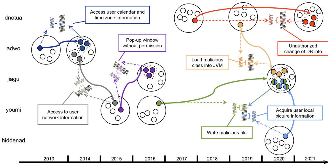
Fig. 12. Genetic knowledge graph of “jiagu” and “adwo”.
