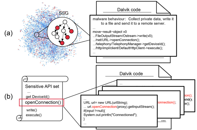
Fig. 10. Advantages of SSG in traceability analysis.
