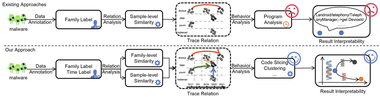
Fig. 1. The novelty demonstration of automated malware traceability analysis.
