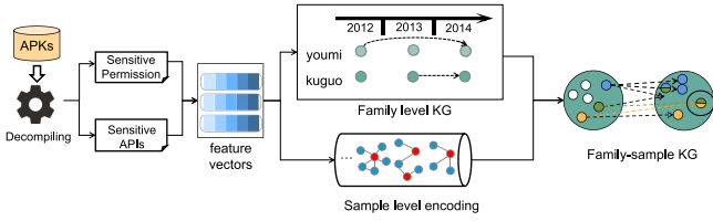
Fig. 4. Knowledge graph construction.
