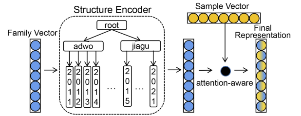
Fig. 6. Hierarchical feature structure.
