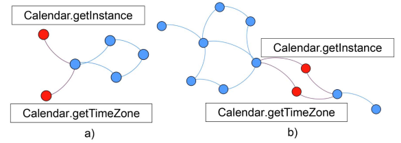
Fig. 9. SSGs in the same cluster.
