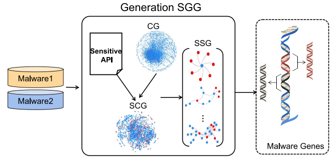
Fig. 3. Workflow of SSG generation.
